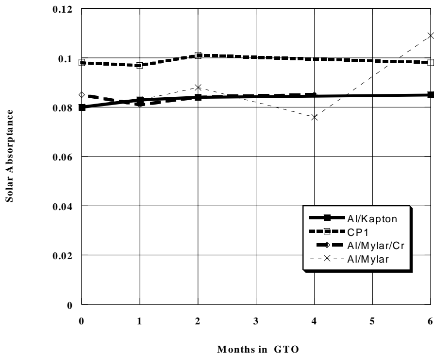
Figure 4. Solar absorptance of the candidate sail materials after exposure to equivalent GTO exposure
