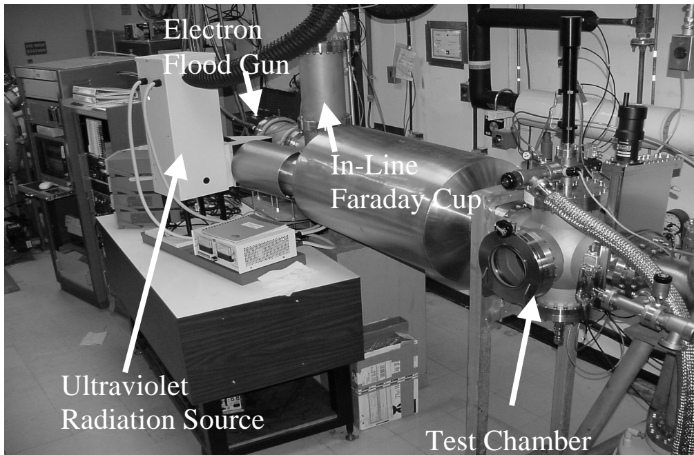
Figure 1. Low Energy Electron (LEE) System at MSFC.
