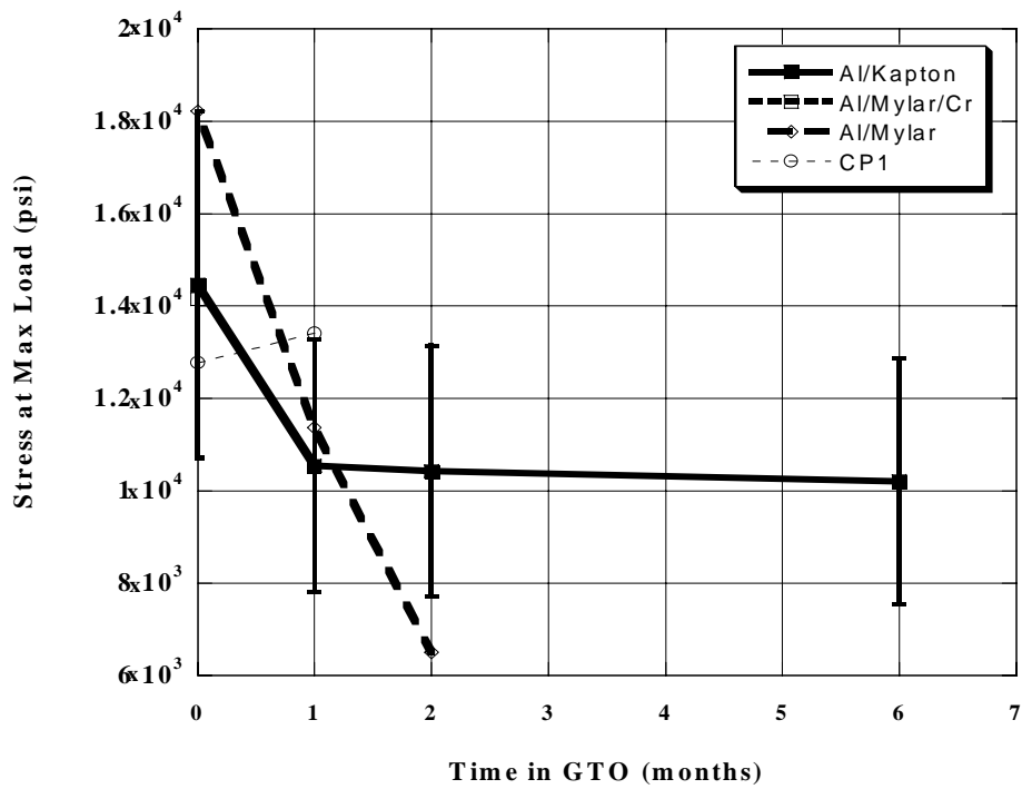
Figure 3. Effects of a simulated GTO dose on the stress of candidate solar sail material
