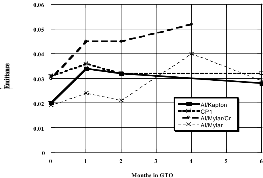
Figure 5. Emittance of the candidate sail materials after exposure to equivalent GTO exposure
