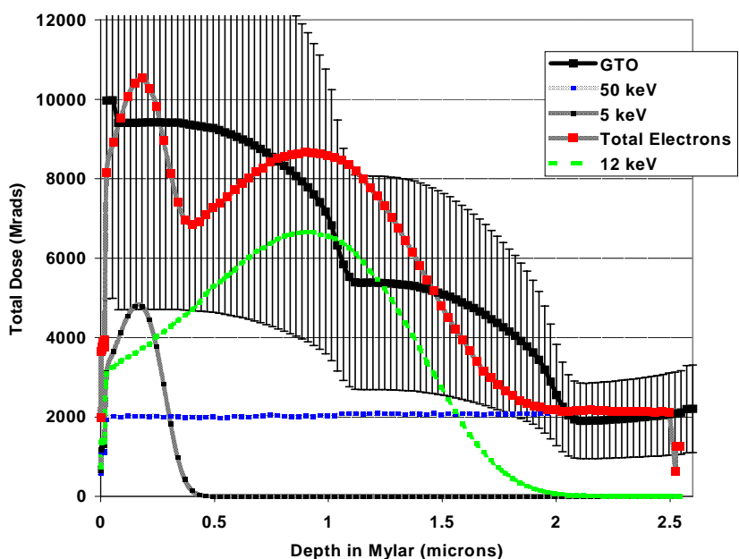
Figure 2. Dose-Depth profile for Mylar in GTO for 1 year.
